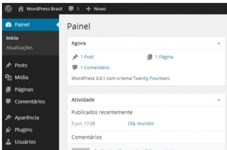
Figura 2: WordPress
